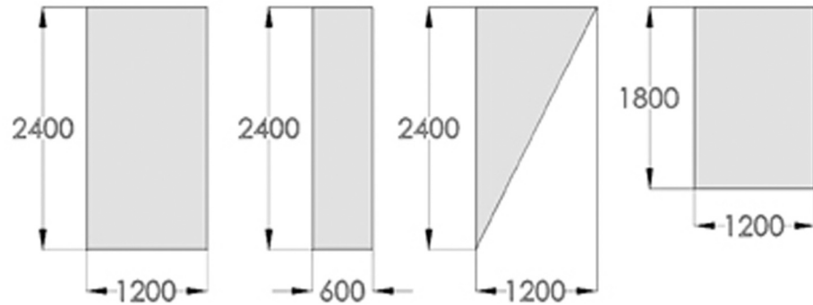
Stage Decking Standard Sizes
